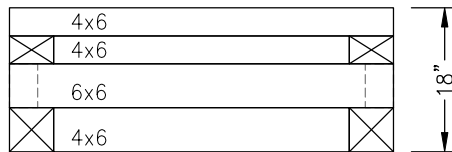
Detail C
